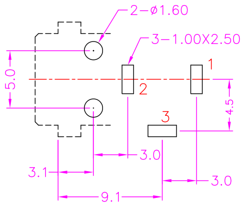
RECOMMEND P.C.B LAYOUT TOP VIEW
