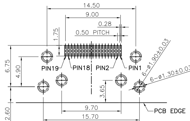
RECOMMEND PCB LAYOUT TOLERANCE: ±0.05(TOP VIEW)
