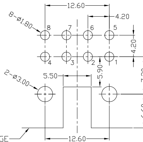
RECOMMEND P.C.B. LAYOUT TOP VIEW TOLERANCE ±0.05 mm
